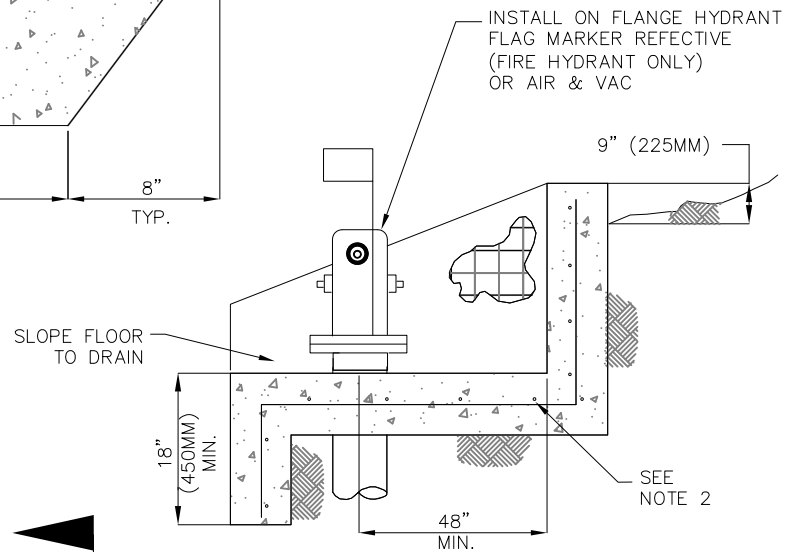
SECTION A-A CONCRETE (OR BLOCK) RETAINING WALL (TO BE USED WHERE GROUND SLOPE EXCEEDS 30% OR AS REQUIRED)
