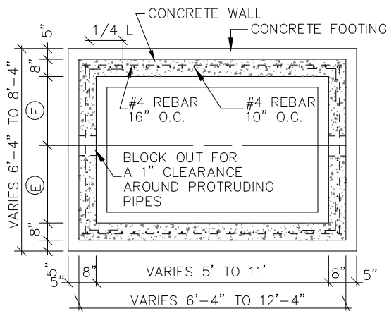
BOX PLAN
