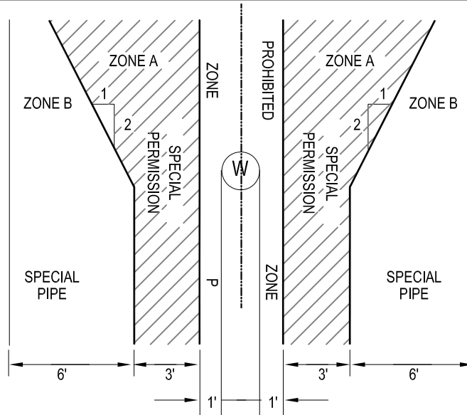
CASE 1 NEW WASTEWATER (SEWER) MAIN
