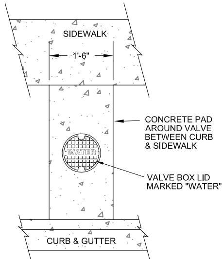
COLLAR FOR VALVES LOCATED IN PARKSTRIP N.T.S.
