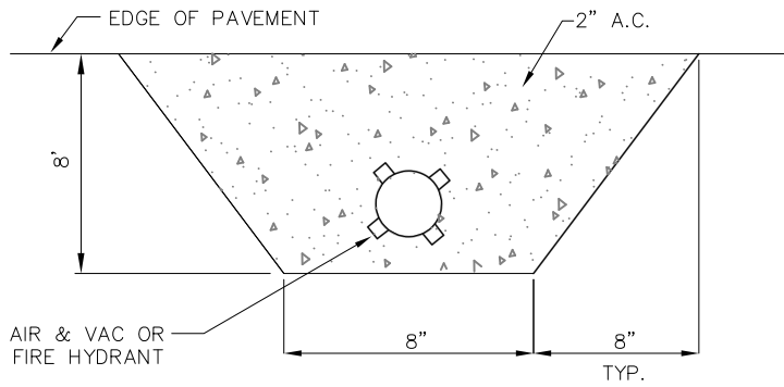
FIRE HYDRANT OR AIR AND VAC IN STREET SHOULDER
