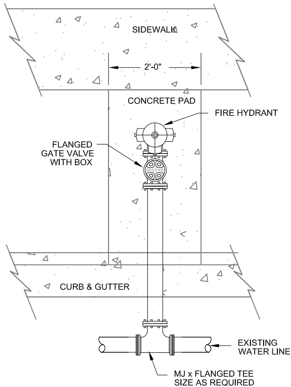
PLAN VIEW
