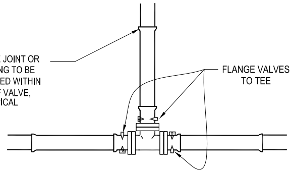
TEE-TYPICAL CONNECTIONS
