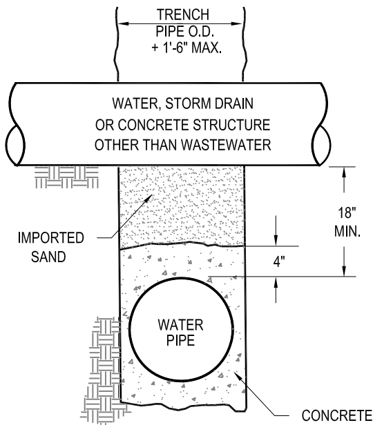
ENCASEMENT NEAR OBSTRUCTIONS (SEE NOTE 3)
