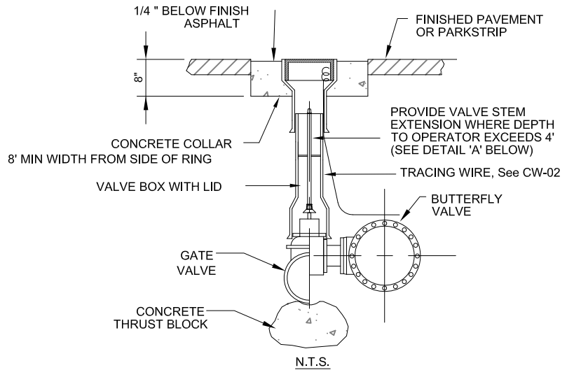
COLLAR FOR VALVES LOCATED IN PARKSTRIP N.T.S.
