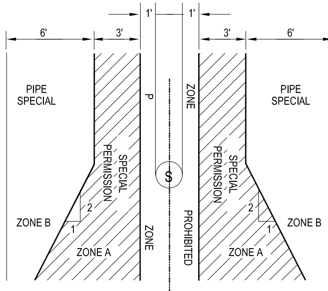
CASE 2 NEW WATER MAIN
