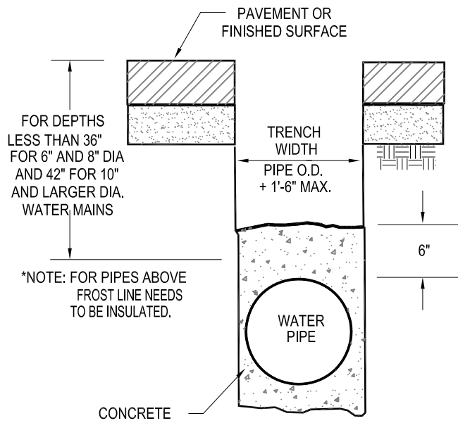
ENCASEMENT FOR COVER LESS THAN MINIMUM (SEE NOTE 4)
