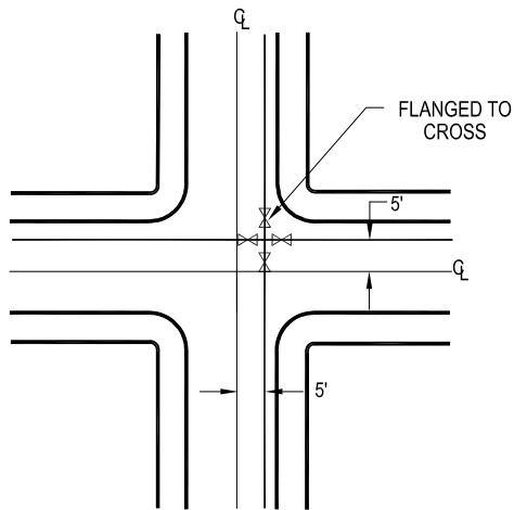
CROSS-TYPICAL CONNECTIONS
