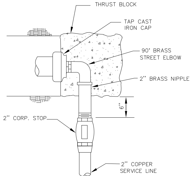
END-OF-MAIN CONNECTION
