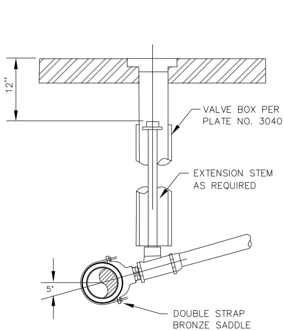
ON-MAIN CONNECTION
