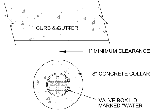
COLLAR FOR VALVES LOCATED IN ROADWAY N.T.S.
