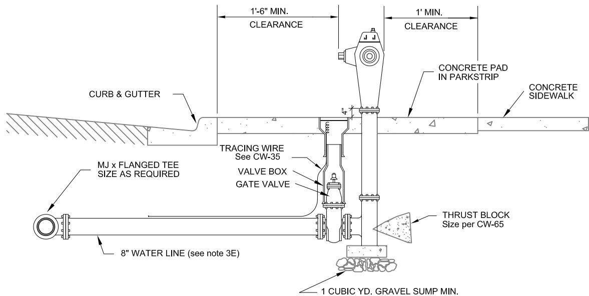
TYPICAL PROFILE
