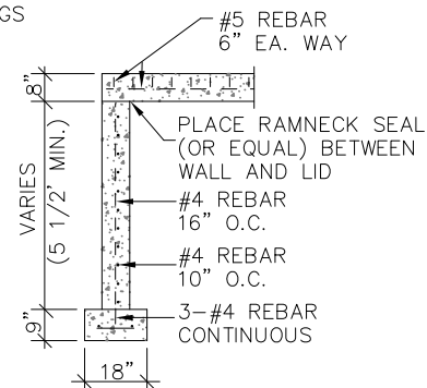
BOX SECTION
