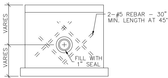
BOX SIDE ELEVATION
