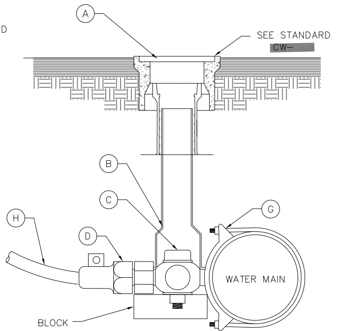
STOP IN ROADWAY
